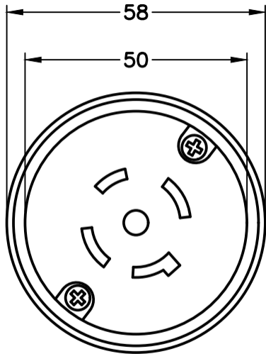
NEMA L21-20 CONNECTOR FRONT VIEW
